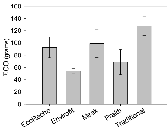
Figure 8: Average Total CO. Error bars are 95% confidence intervals. From left to right, the values are: 92.7 \pm 16.7 , 54.1 \pm 4.3 , 99.0 \pm 22.9 , 69.0 \pm 20.4 , 127.6 \pm 15.5 .
