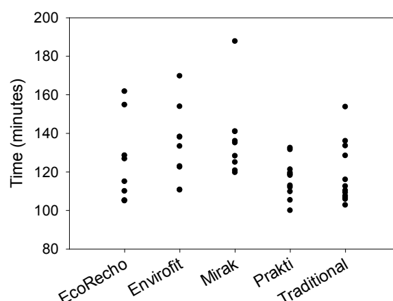
Figure 5: Total Burn Time per test. See Appendix B for specific values.
