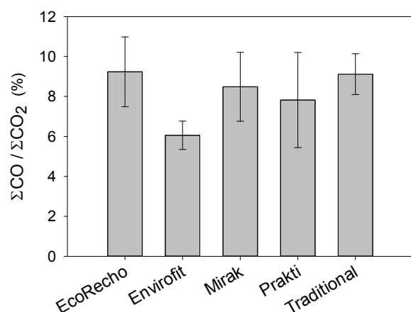
Figure 12: Average Ratio of CO/CO 2 (%). Error bars are 95% confidence intervals. From left to right, the values are: 9.2 \pm 1.7 , 6.1 \pm 0.7 , 8.5 \pm 1.7 , 7.8 \pm 2.4 , 9.1 \pm 1.0 .
