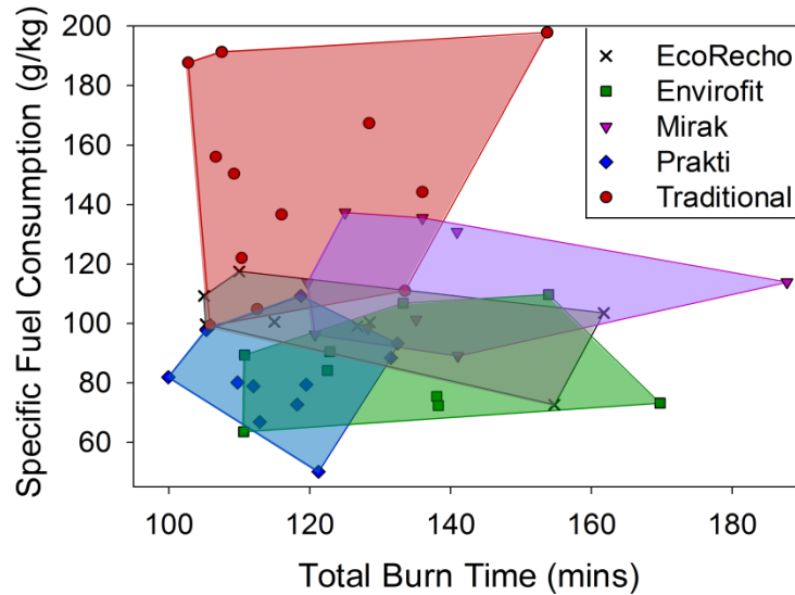
Figure 8: Correlation between Total Burn Time and Specific Fuel Consumption. Shading indicates the convex polygon containing all data points from our tests, not necessarily all potential data points.
