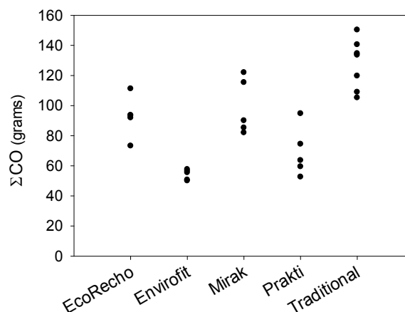
Figure 9: Total CO per test. See Appendix C for specific values.
