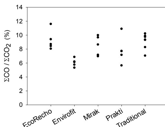
Figure 13: Ratio of CO/CO 2 per test (%). See Appendix C for specific values.
