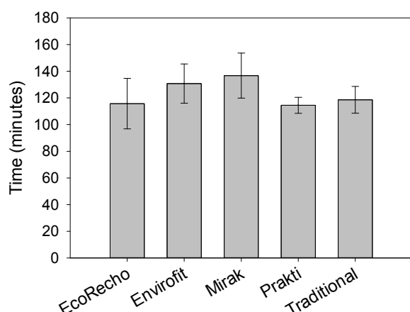
Figure 4: Average Total Burn Time. Error bars are 95% confidence intervals. From left to right, the values are 115.7 \pm 18.9 , 130.8 \pm 14.7 , 136.7 \pm 16.9 , 114.5 \pm 6.0 , 118.6 \pm 10.0 .
