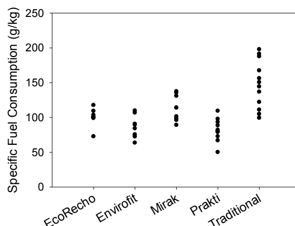
Figure 7: Specific Fuel Consumption per test. See Appendix B for specific values.
