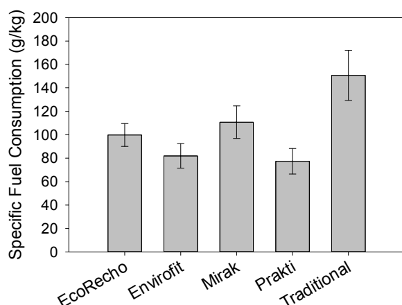
Figure 6: Average Specific Fuel Consumption. Error bars are 95% confidence intervals. From left to right, the values are: 99.8 \pm 9.7 , 81.9 \pm 10.5 , 110.7 \pm 13.8 , 77.4 \pm 10.9 , 150.7 \pm 21.4 .
